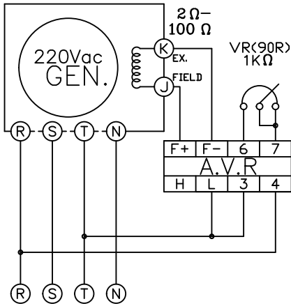
GEN 220V connection
