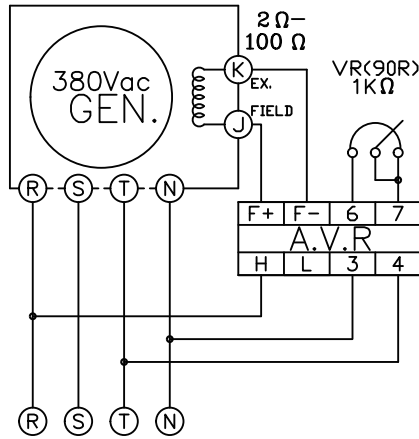
GEN 380V connection
